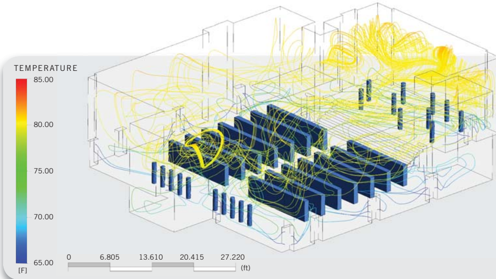
LEFT CFD SAMPLE RESULTS OF A LIBRARY USING DISPLACEMENT VENTILATION.
